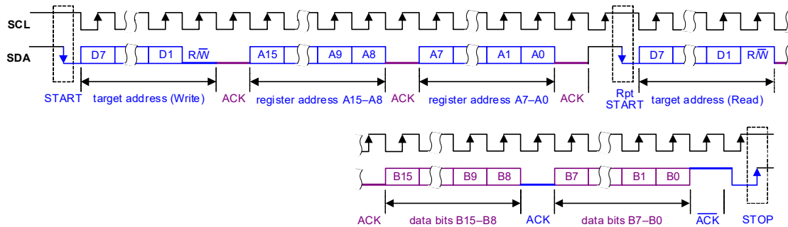
Figure 4-33. Control Interface I 2 C Register Read
